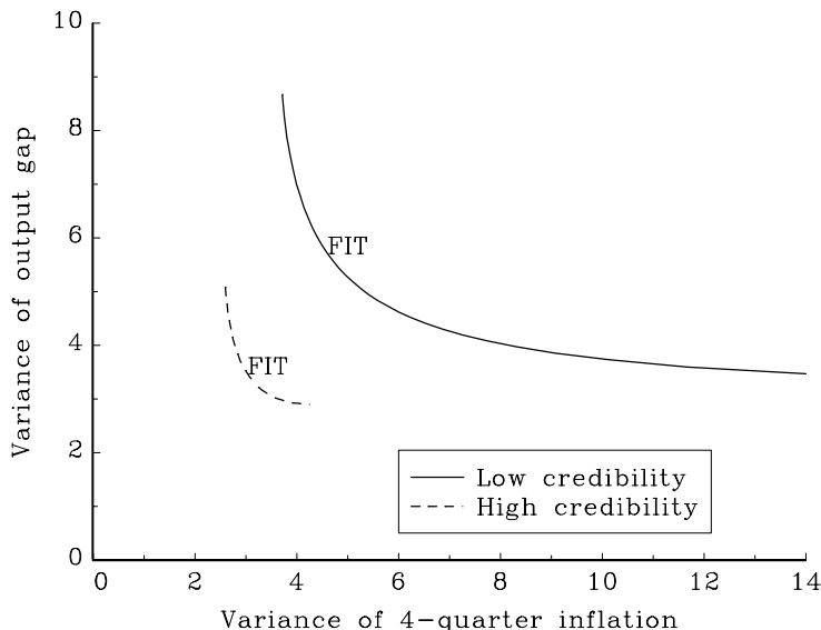
Figure 4.2: Variance tradeoffs for low and high credibility, United States
