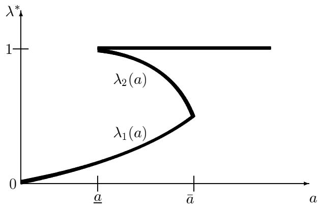
Figure 2.2: Case \beta_1 < \beta < \beta_2
