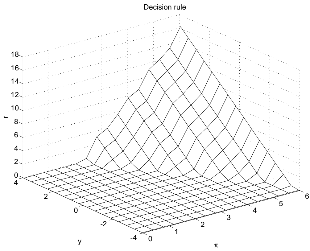
Figure 6: A plot of the decision rule, using \pi^* = 2 and \lambda = 1 .
