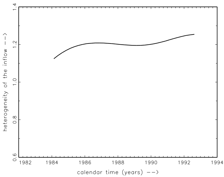
Figure 4: The estimated cyclical variation of the indicator of the compositional changes in the inflow.
