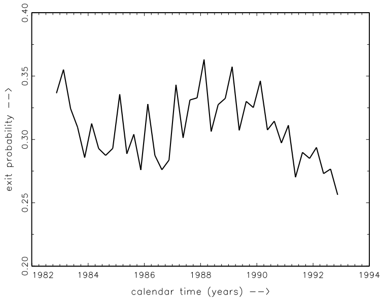
Figure 1: The quarterly over-all exit probability in the macro data.
