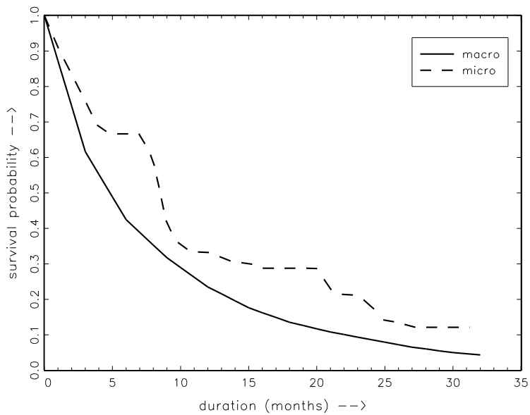
Figure 2: Kaplan-Meier estimate of the outflow in the micro and the macro data of individuals who were unemployed in June 1990 for less than 3 months.
