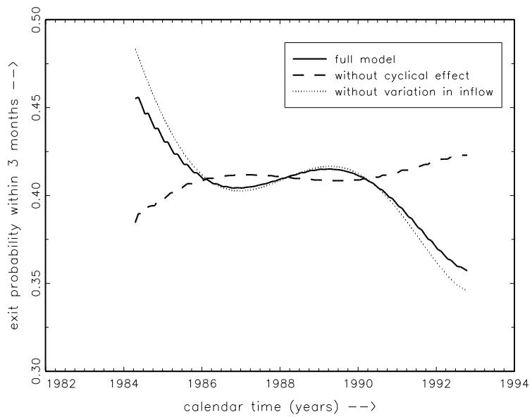
Figure 5: The estimated probability of leaving unemployment within 3 months.
