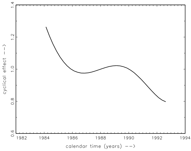
Figure 3: The estimated cyclical variation of the individual exit probability ( \psi_{2,b}(\tau) ).
