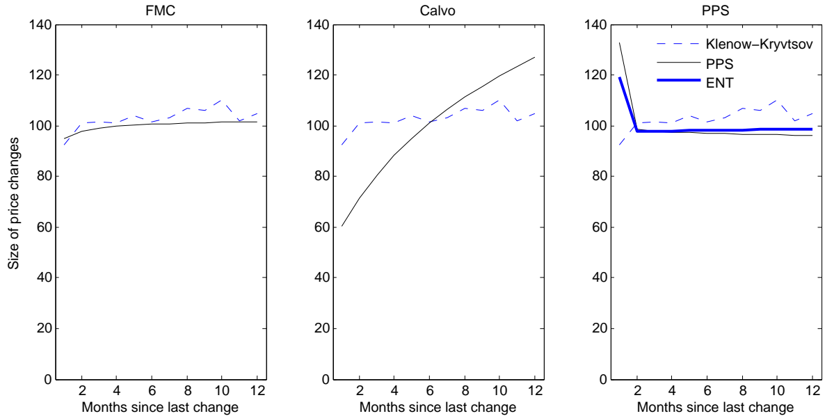
Fig. 5. Mean adjustment and price duration: comparing models
