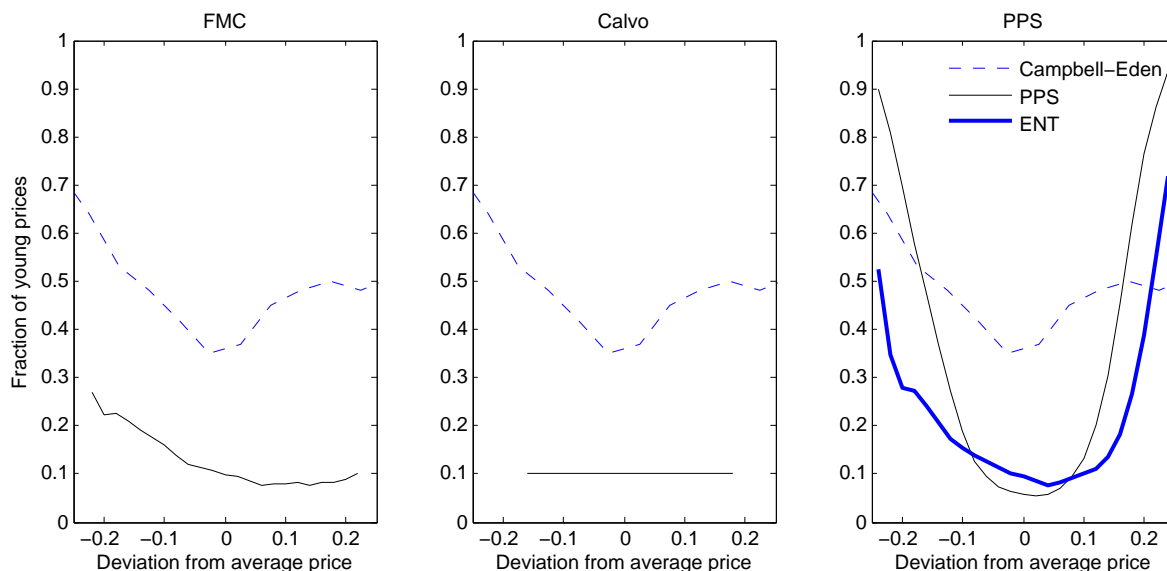
Fig. 6. Extreme prices tend to be young: comparing models
