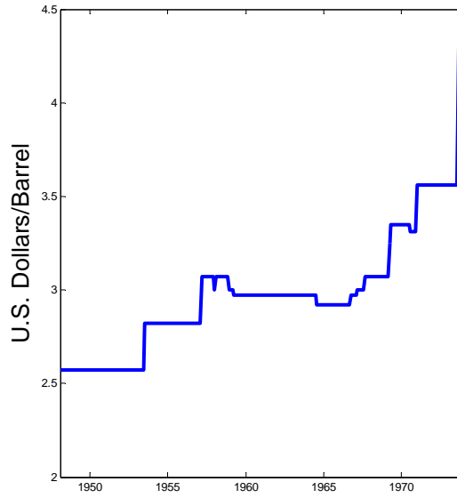
Figure 1. Price of West Texas Intermediate Crude Oil: 1948.1-1973.12
