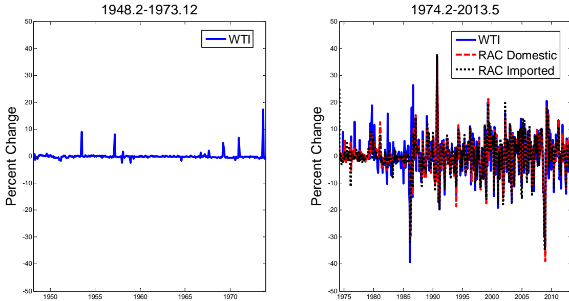
Figure 2. Percent Change in the Real Price of Oil
