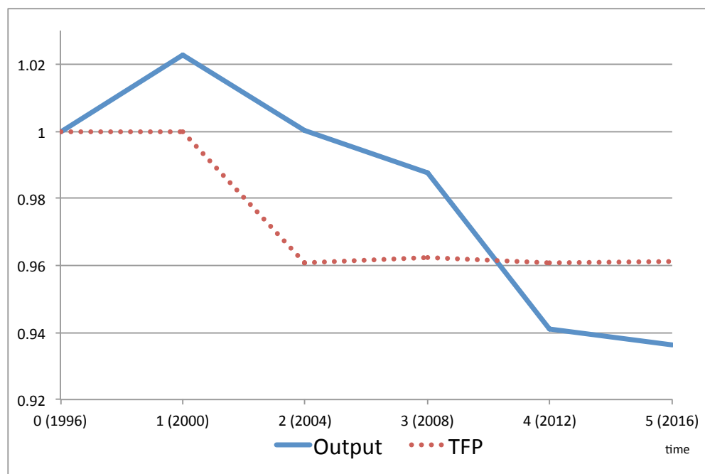
Figure 5: Boom, Slump and Crash in the Model After a Series of Financial Shocks
