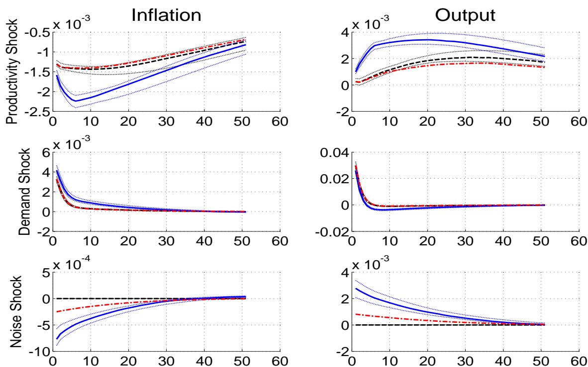
FIGURE 2. Posterior impulse response functions. Blue solid lines are for man-bites-dog signal available in impact period and black dashed lines for no man-bites-dog signal. Dotted lines show the 95 per cent posterior credible intervals. The dash-dot red lines are the responses of inflation and output when the availability of the signal z_t^a is uncorrelated with the innovation to productivity.
