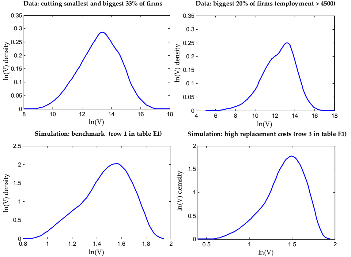
Figure 9: Distribution of \ln V – simulation and data
