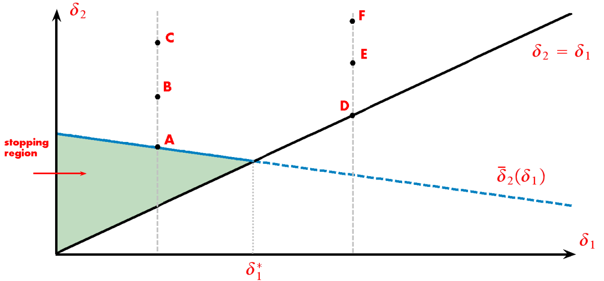
Figure 3: Optimal Policy
