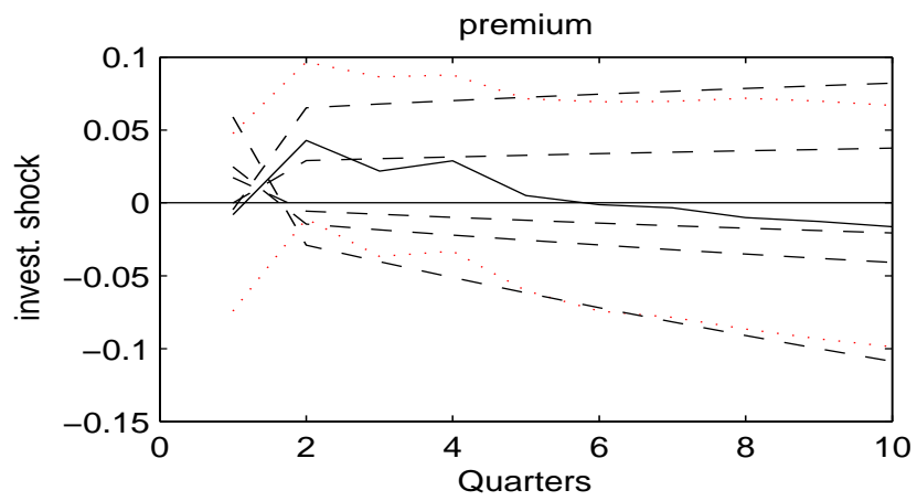
Figure 8: Capital-skill substitutability
