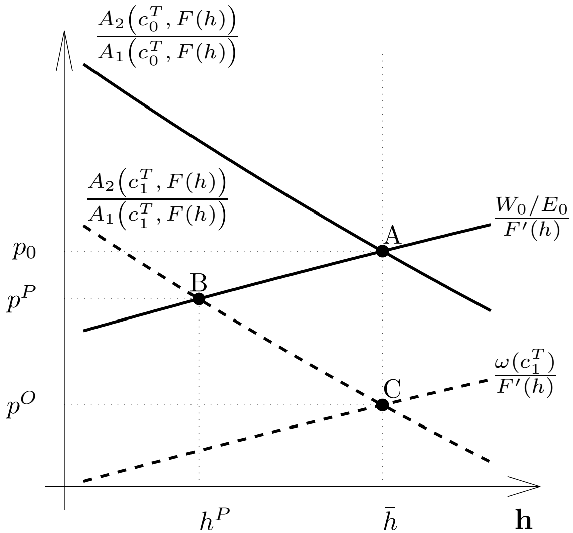
Figure 2: General Disequilibrium
