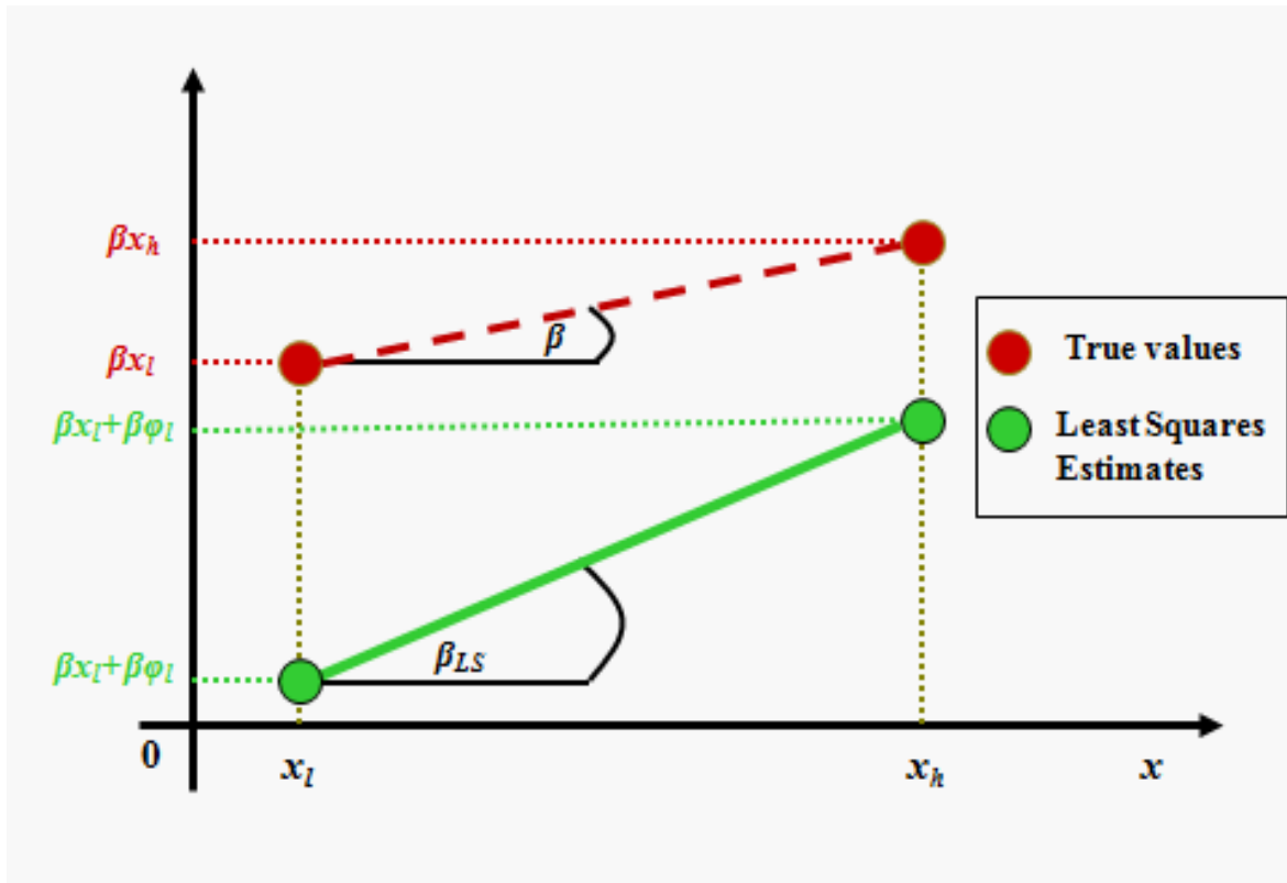
Figure 1: Illustrating the LS Amplification Bias
