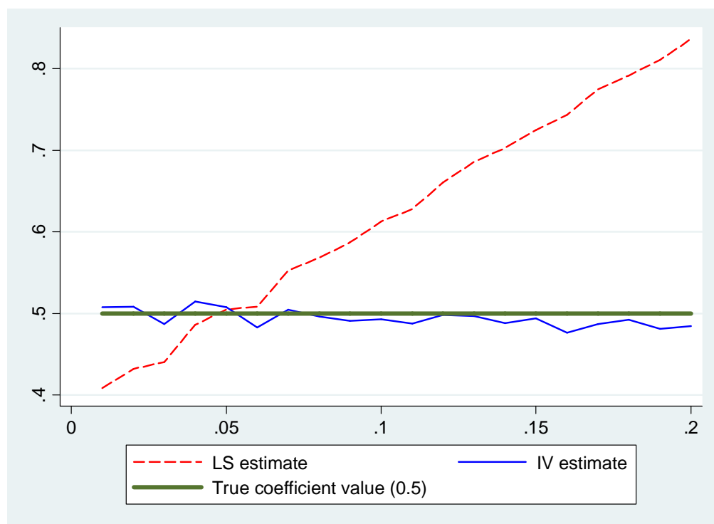
Figure 3: Monte Carlo Simulation Comparing the LS and the IV Estimate
