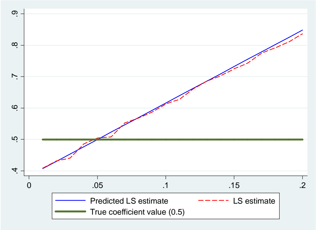
Figure 2 plots the bias of the standard cross-industry cross-country estimator in a Monte Carlo simulation (on the vertical axis) for different values of \sigma (on the horizontal axis) in (14). The dashed red line is the average least-squares (LS) estimate from the Monte Carlo simulation. The solid blue line is the asymptotic bias implied by equation (15). The true parameter value is 0.5. See the Sub-Section entitled "Amplification and Attenuation Bias in a Simple Example" in Section 2.2.1 for an explanation.
