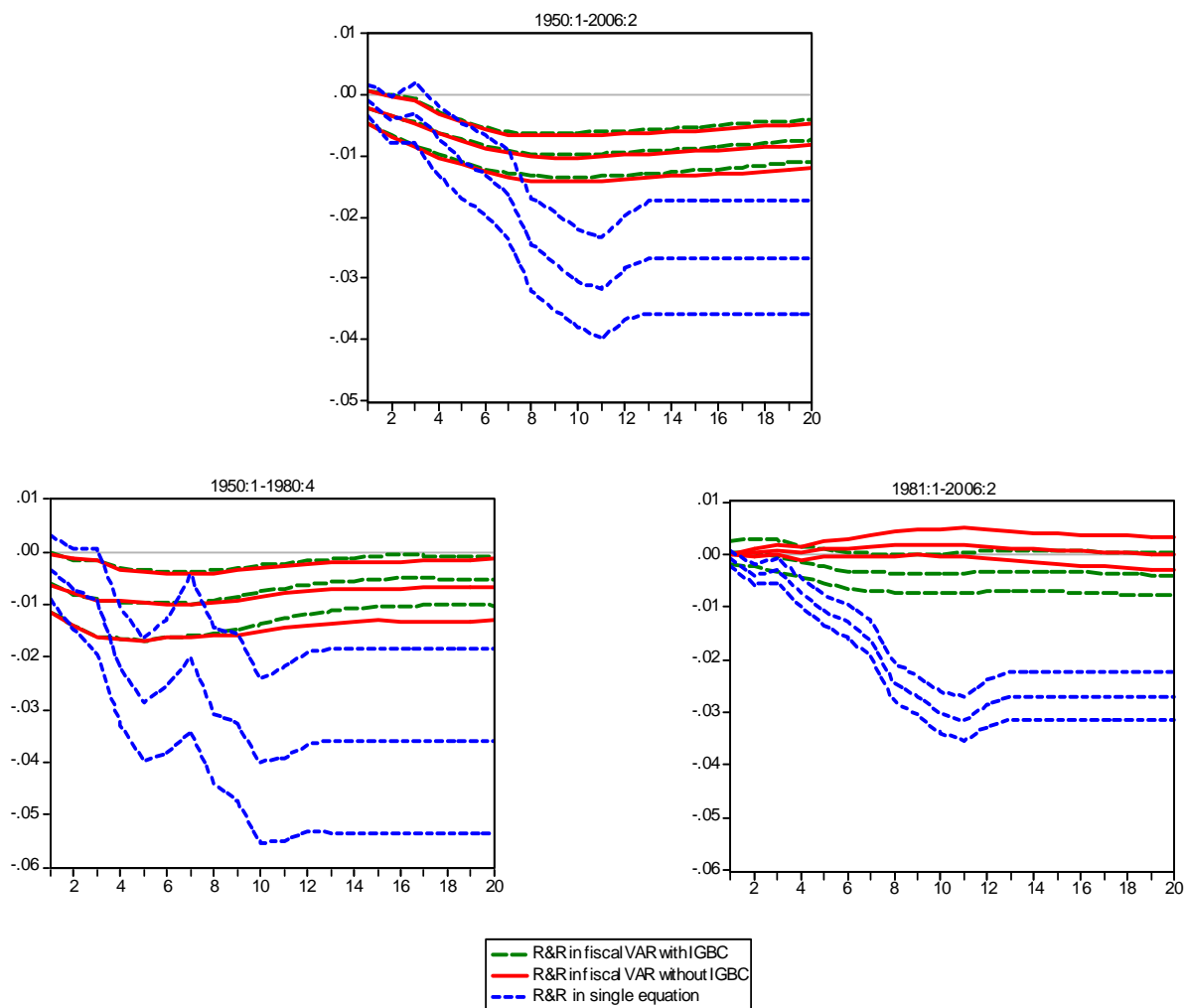
Figure 4: Estimated Impact of an Exogenous Tax Increase of 1% of GDP on GDP: R&R single equation approach (dots), Fiscal VAR with (interrupted lines) and without (continuous line) the government intertemporal budget constraint
