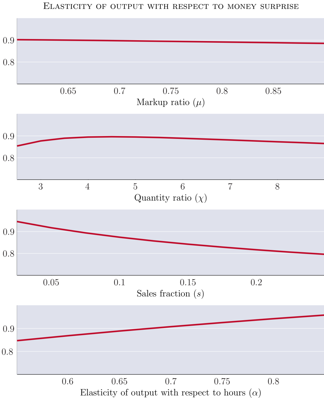
Figure 5: Sensitivity analysis
