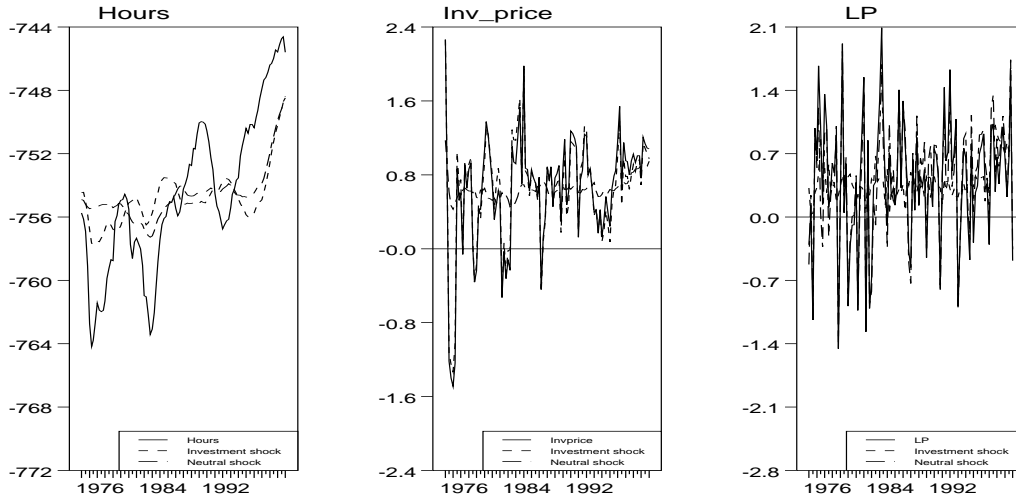
Figure 11: Historical decomposition
