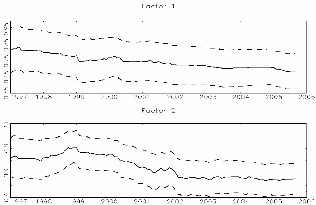
Figure 11: Recursive persistence of factors, Euro area, sample 1991 – 2005
