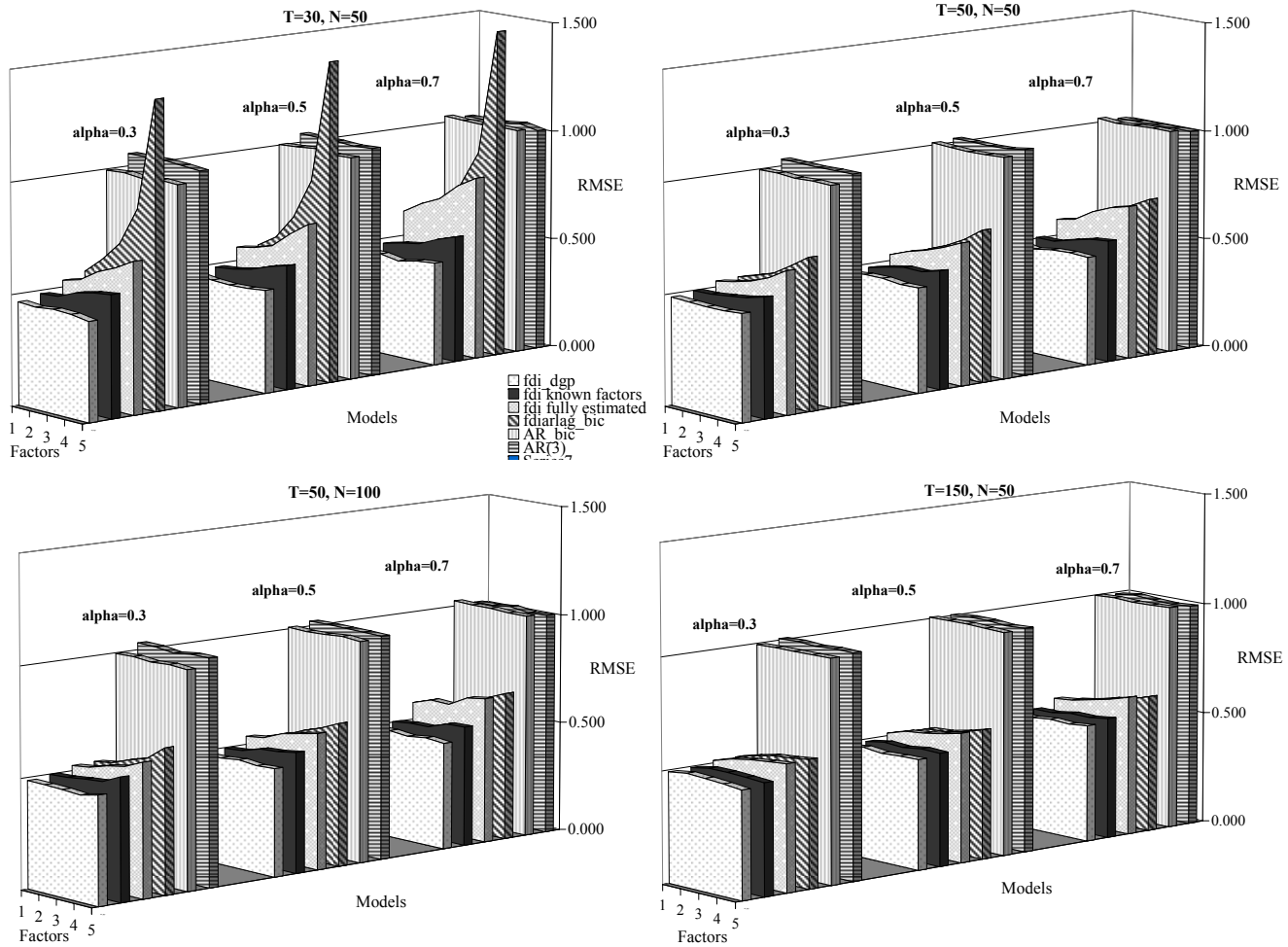
Figure 1: Basic DGP, h = 1
