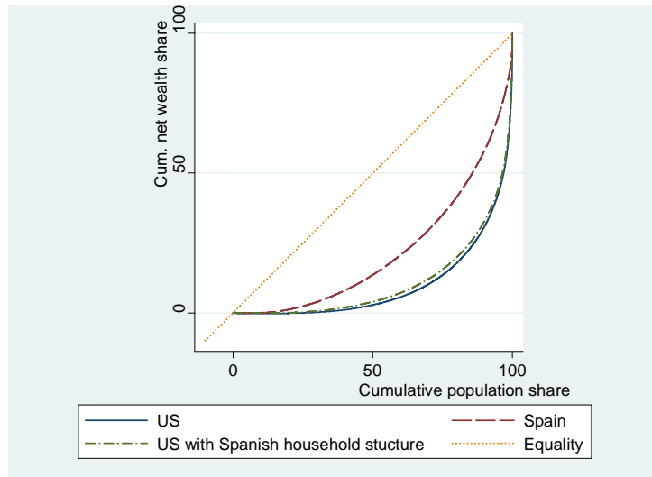
Figure 3: Lorenz curves
