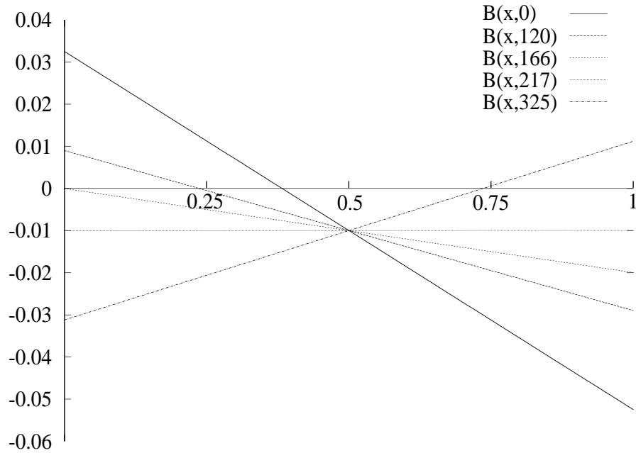
Figure 1: Risk Aversion and Oligopolistic Reaction
