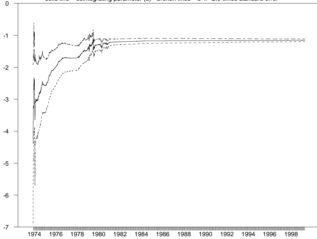
Figure 1: Recursive estimate of the cointegrating parameter
