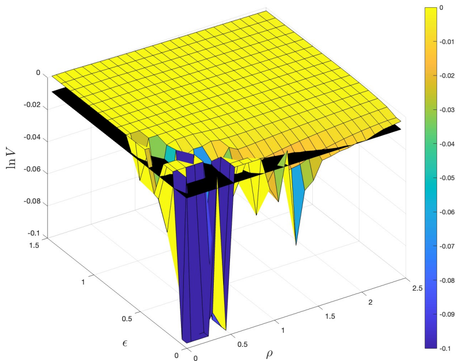
(a) Simulated \ln V_t vs. HOTA implied approximation for German Chemicals
