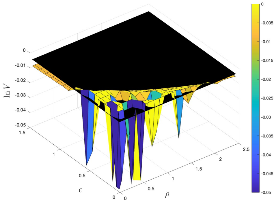
(b) Simulated \ln V_t vs. SHOTA implied approximation for Russian Petroleum
