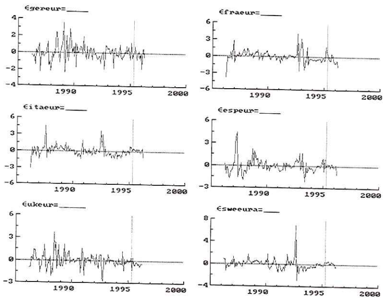
Figure 4: Modelling European Central Banks reaction functions: the difference between actual and fitted short-term interest rates
