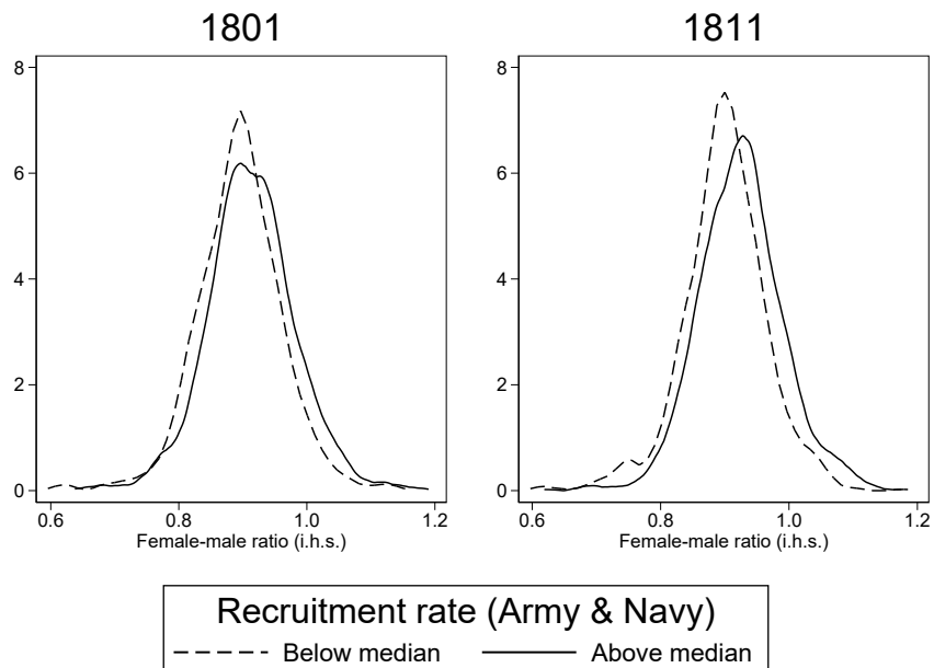
Figure A.2: Sex Ratios and Recruitment
