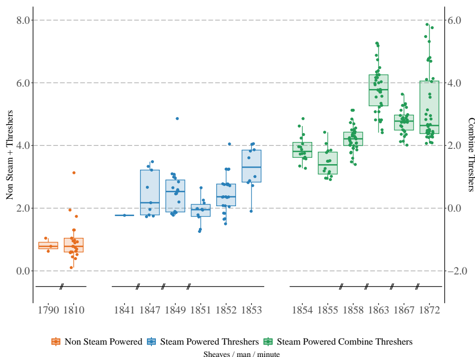
Figure 2: Productivity of threshing machines: 1790-1872
