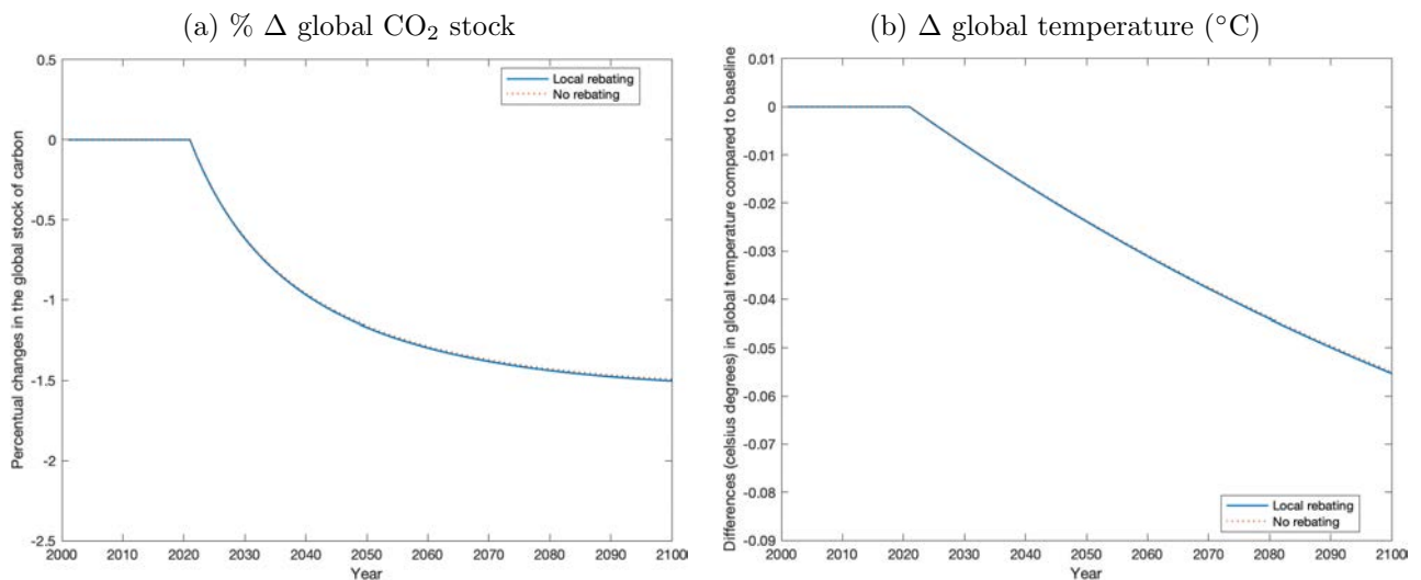
Figure D4: Effect of Different Rebating Schemes of US Carbon Tax on Global CO 2 Stock and Temperature
