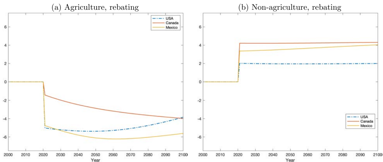
Figure 24: Change in Sectoral Output due to US Carbon Tax (Local Rebating), Select Countries
