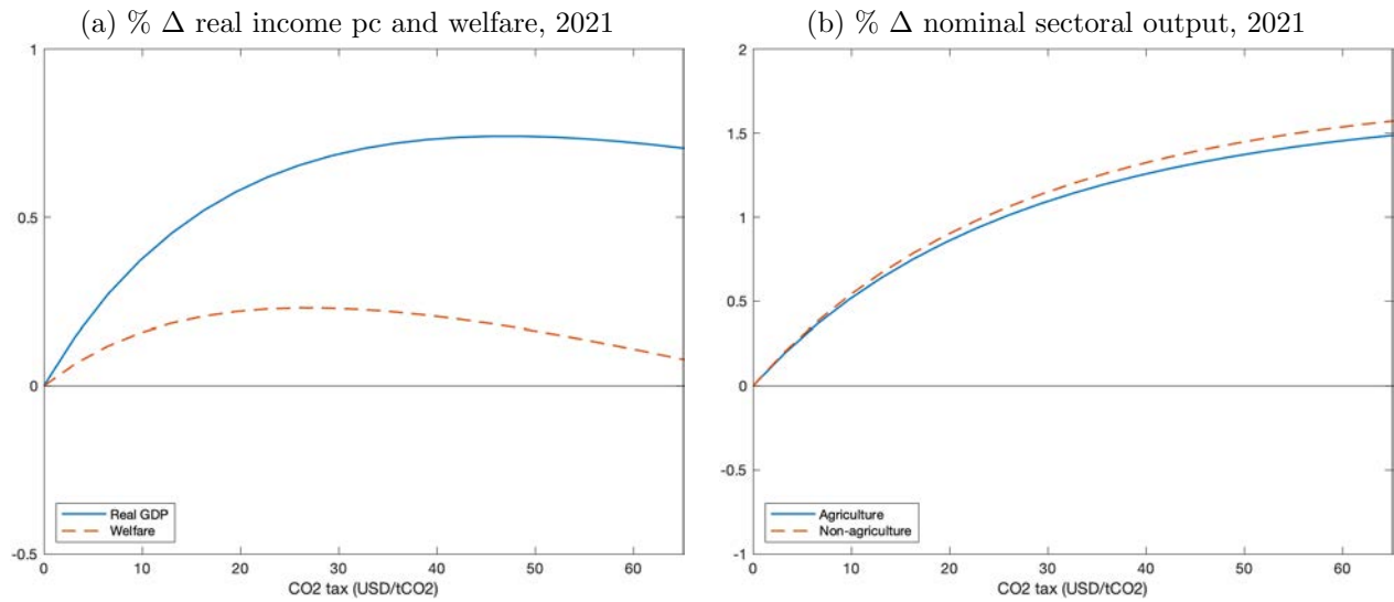
Figure 26: Effect of US Carbon Tax on World Economy (Local Rebating), 2021
