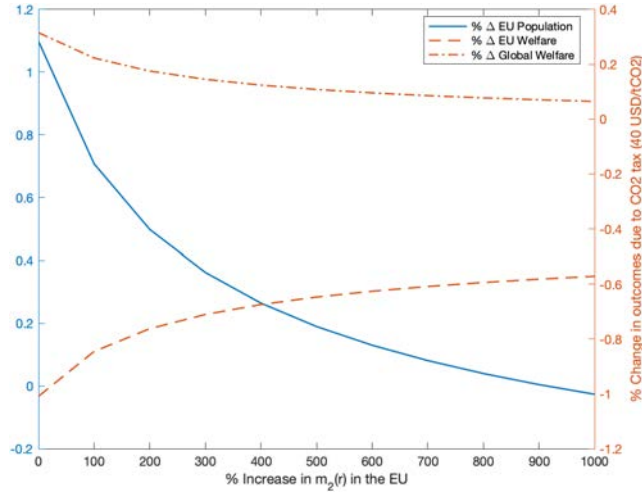
Figure 15: Effect of Carbon Tax on EU for Different Migration Costs (Local Rebating), 2021
