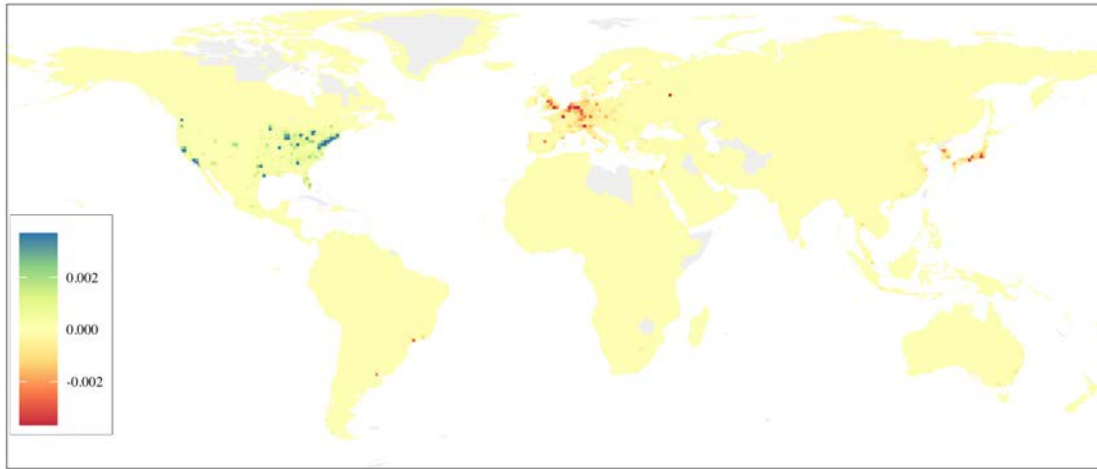
Figure D3: Effect of US Carbon Tax on Emissions around the World (Local vs No Rebating), 2021
