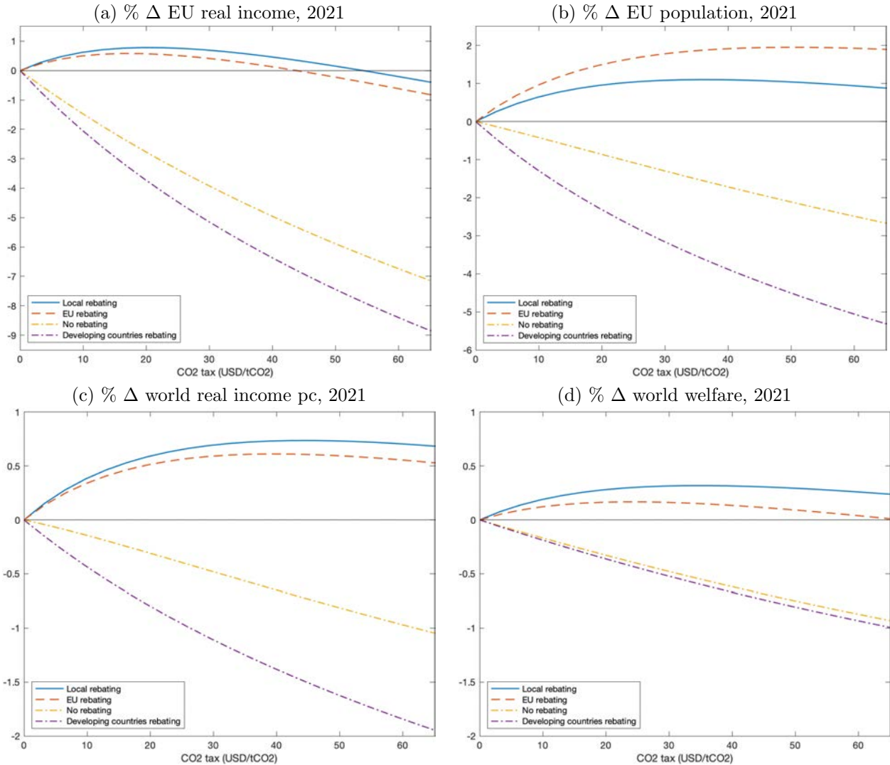
Figure 18: Effect of Different Rebating Schemes on EU and World Economy, 2021
