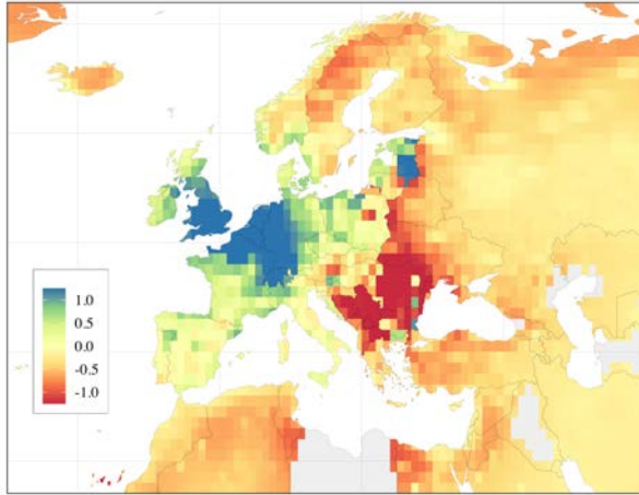
(a) % \Delta agr., EU – local rebating, 2021
