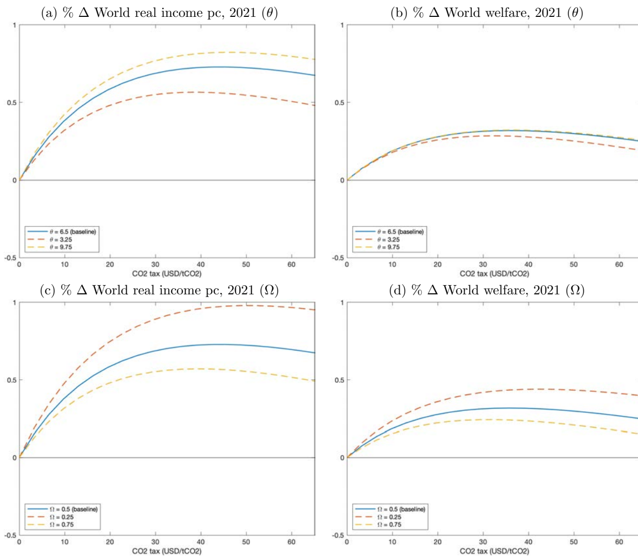
Figure C4: Effect of Different \theta and \Omega on World Outcomes with Local Rebating, 2021
