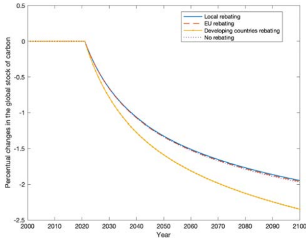
(a) % \Delta global CO 2 stock
