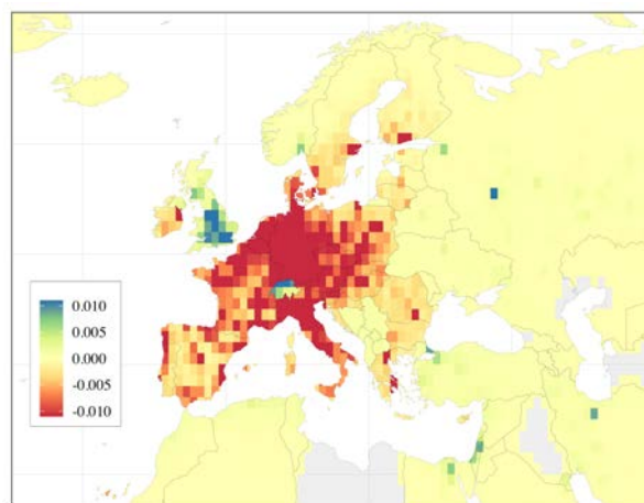
Figure C3: Change in Emissions in the EU Due to Carbon Tax (No Rebating), 2021
