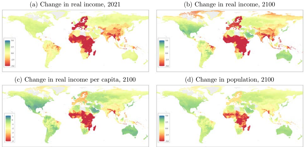
Figure 5: Effect of Carbon Tax on Real Income and Population across the Globe (No Rebating)
