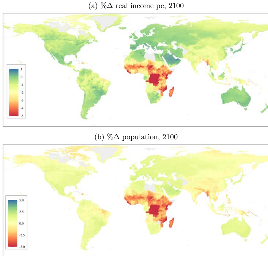
Note: Map displays log difference (*100) in 2100 between the baseline with carbon taxes (and local rebating) and a counterfactual without carbon taxes. Panel (a) shows real income per capita and Panel (b) shows population.
