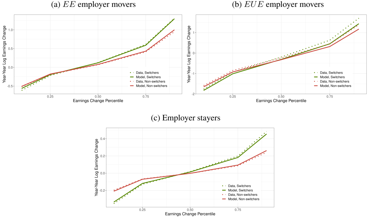
Figure 6: Model fit for the conditional cross-sectional earnings growth distributions (cdf)
