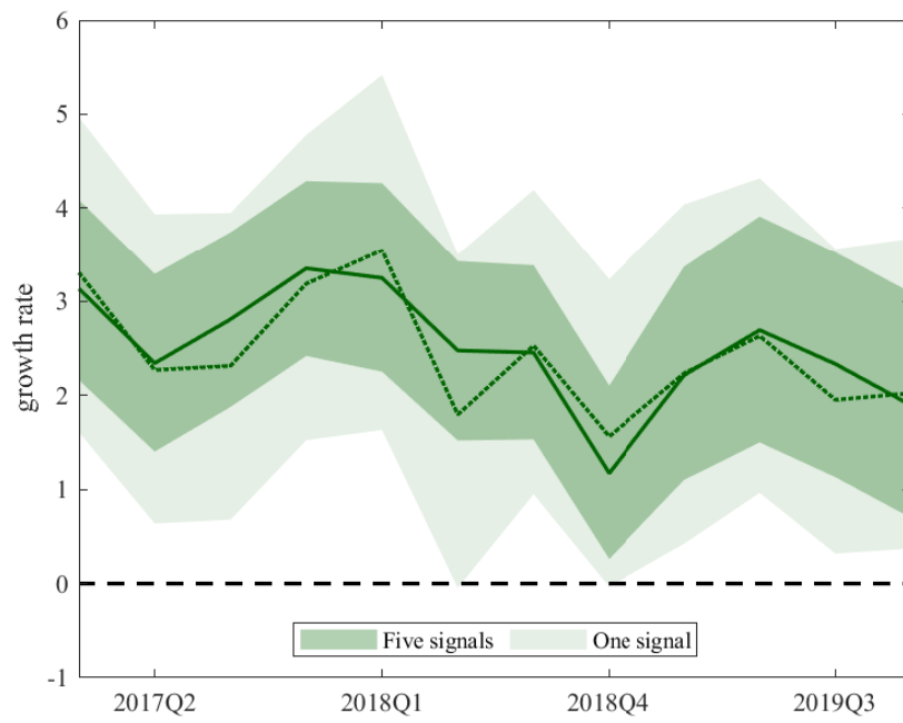
FIGURE 4. Signal extraction for \Delta x_{C_t} . The solid line is the median of \Delta x_{C_t} given y_{1:T} when all signals are used while the dashed line refers to its conditional median when only the most recent signal is used. Shaded areas represent point-wise 90%-probability intervals.
