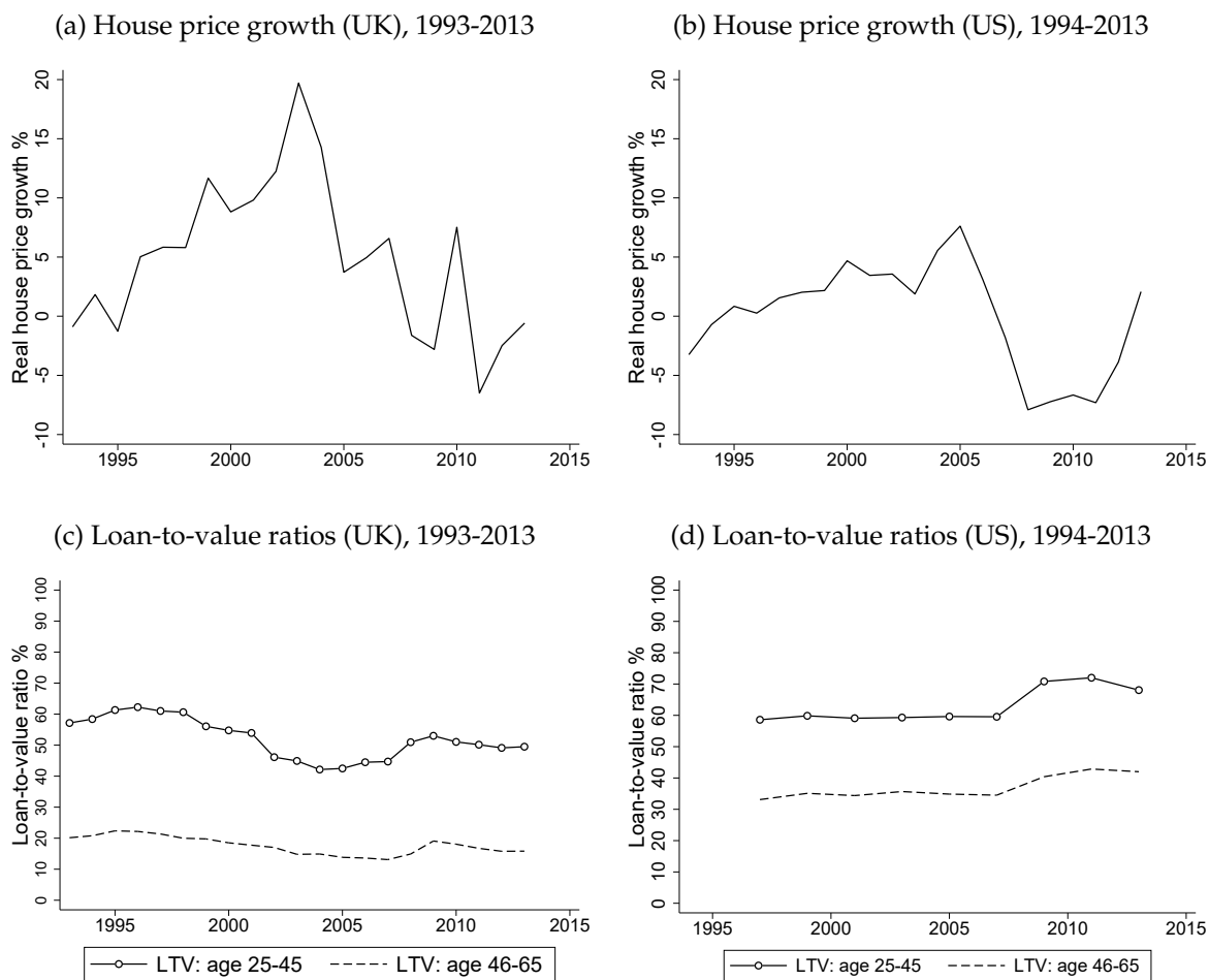
Figure 4: LTV ratios and house price growth rates
