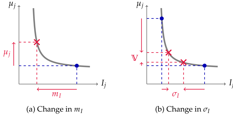
Figure 5: Identification of parameters in category “II. Market”
