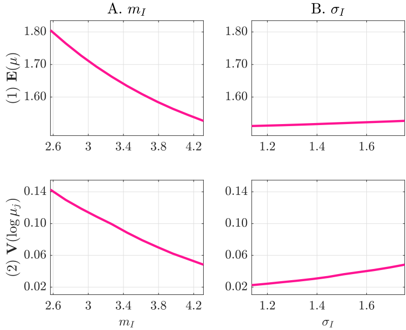
Figure C.4: Comparative static: II. Market
