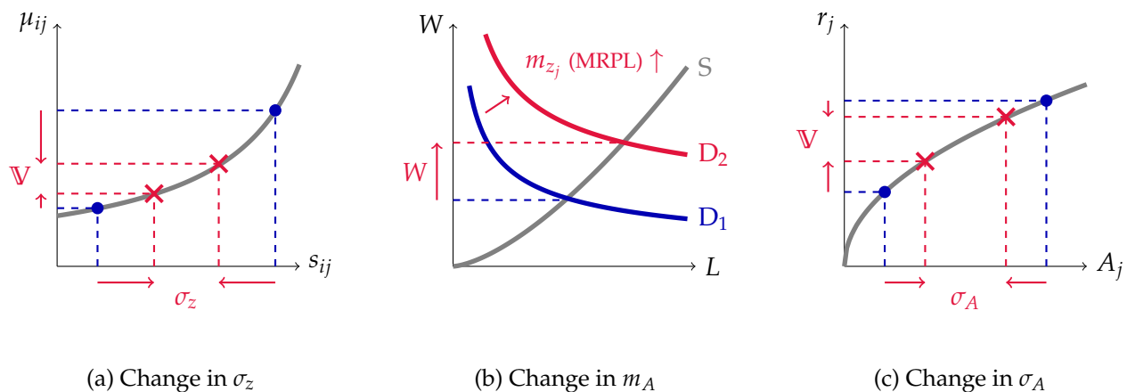
Figure 6: Identification of parameters in category “III. Firm”
