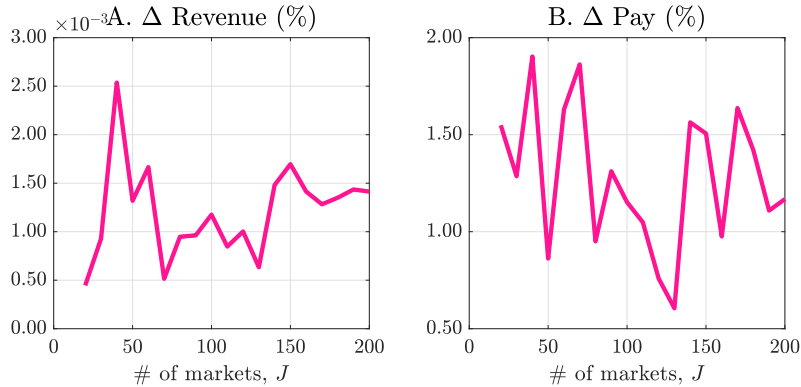
Figure C.2: Robustness of Approximate Stable Matching over J
