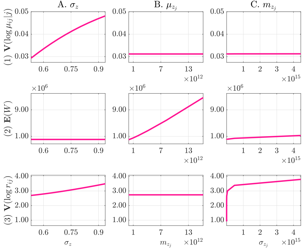
Figure C.5: Comparative static: III. Firm [NOTATION]
