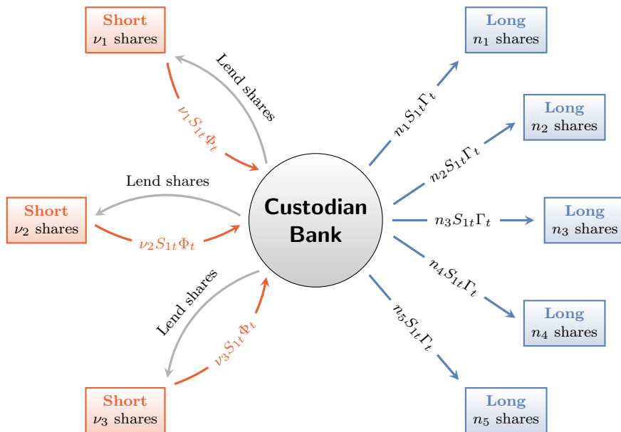
Figure 1: The shorting mechanism. In this example, the short interest in asset 1 amounts to \nu = \sum_i \nu_i \geq 0 shares while the aggregate long position is equal to \sum_k n_k = 1 + \nu shares. As a result, the equilibrium lending yield is \Gamma_t = \frac{\nu}{1+\nu} \Phi_t .
