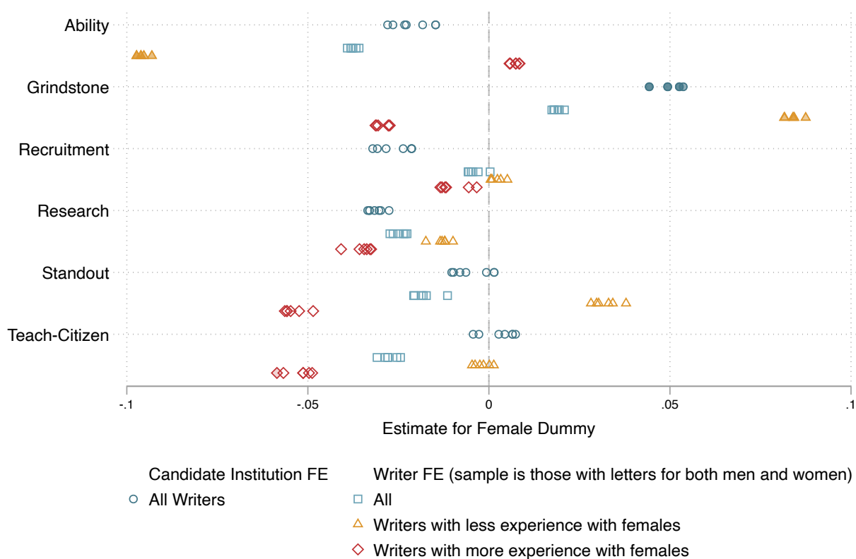
Figure 9: Regression results with candidate institution or writer fixed effects
