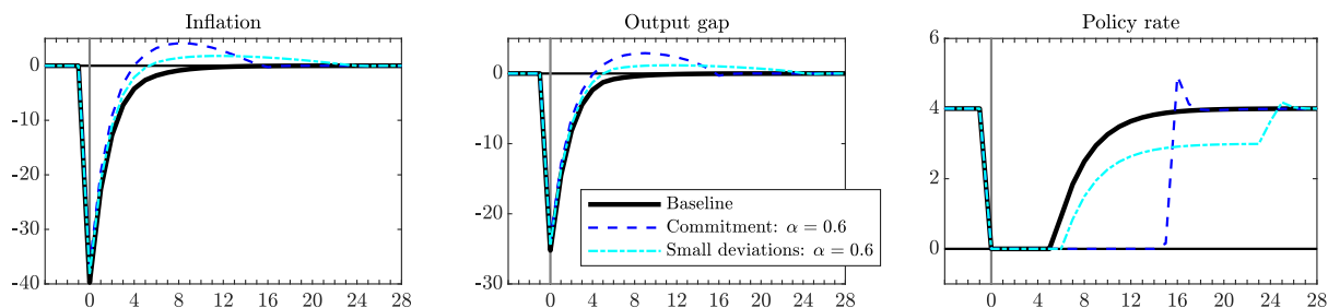
Figure C.3: Commitment + Small deviations + Type I ( \alpha = 0.6 )
