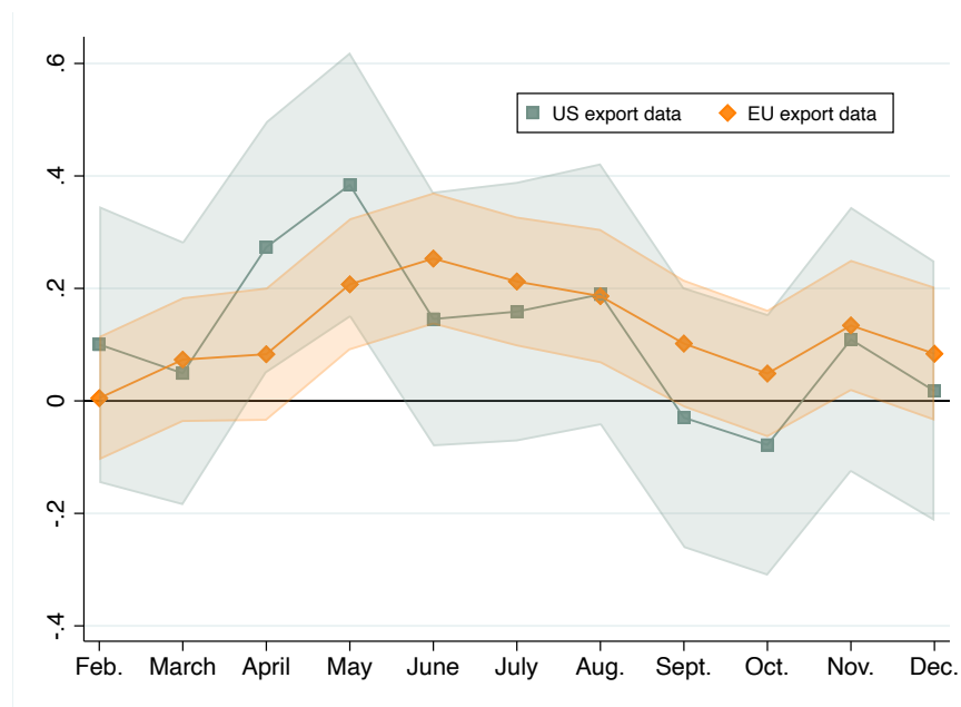
Figure 4: Equation 2 - \beta coefficients, by months of 2020
