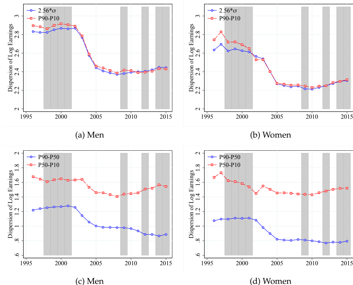
Figure 4: Earnings Inequality
