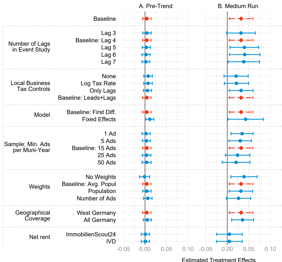
Figure 7: Robustness Checks
