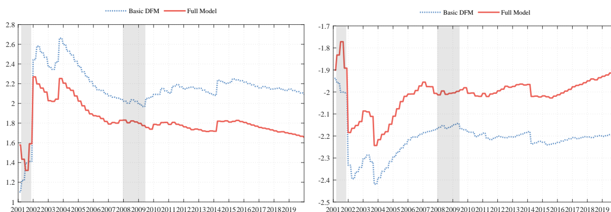
(b) Density forecast accuracy: Log score
