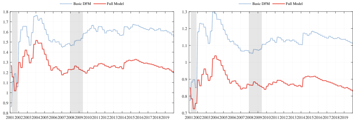
(a) Point forecast accuracy: MAE (b) Density forecast accuracy: CRPS
