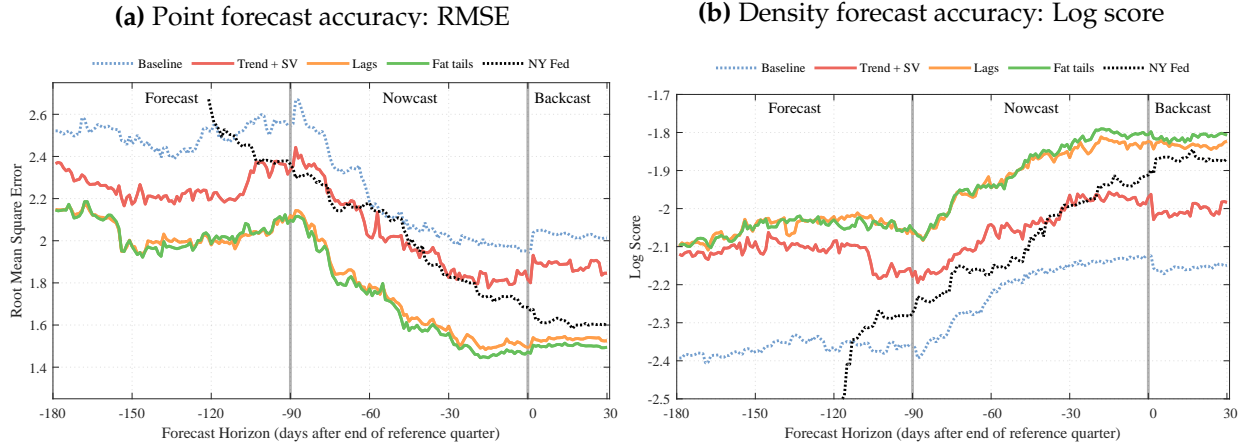
Figure E.5: MODEL COMPARISON AS THE DATA ARRIVES
