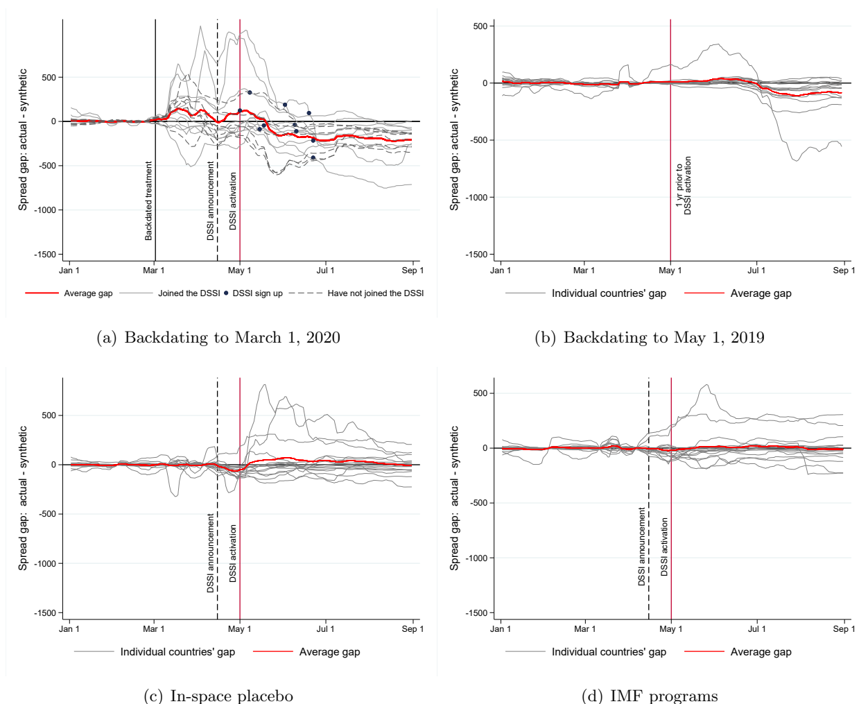
Figure 2: Sovereign bond spreads in DSSI-eligible countries vs their synthetic controls: falsification tests
