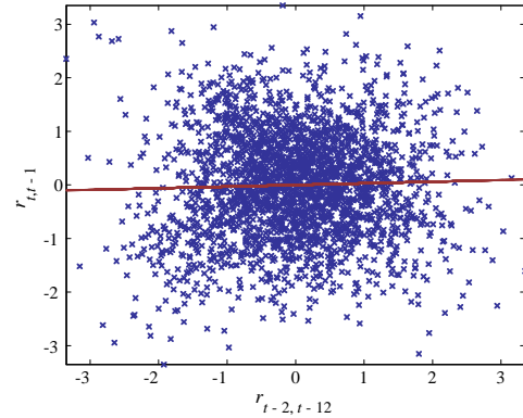
Figure 1f: MOM, Gaussian ranks
