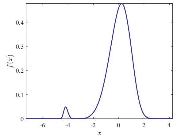
Figure 9d: Mixture of Weibulls density
