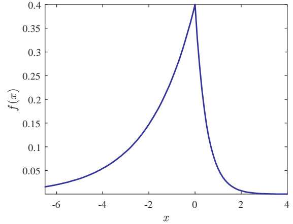
Figure 9d: Mixture of Weibulls density
