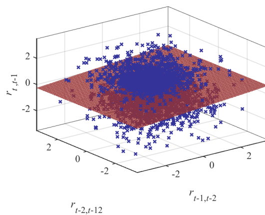
Figure 2c: Gaussian ranks
