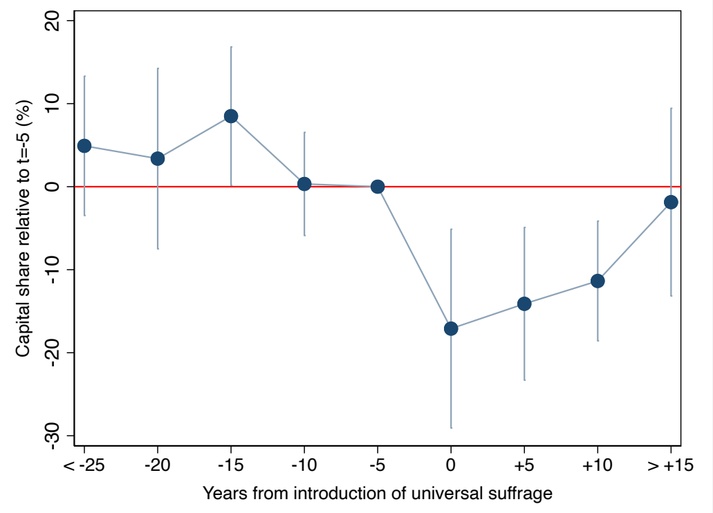
Figure 2: The impact of universal suffrage reform on capital share
