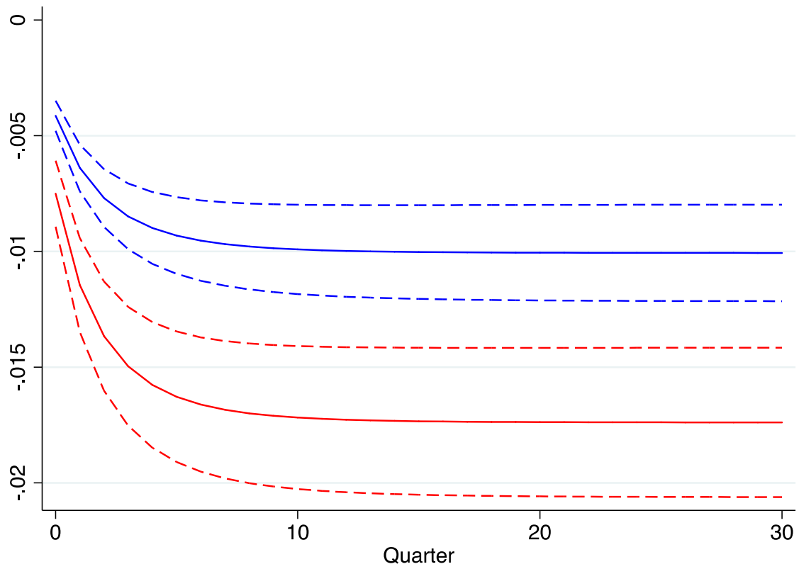
Figure 6: Dynamics of Direct and Global Elasticities
