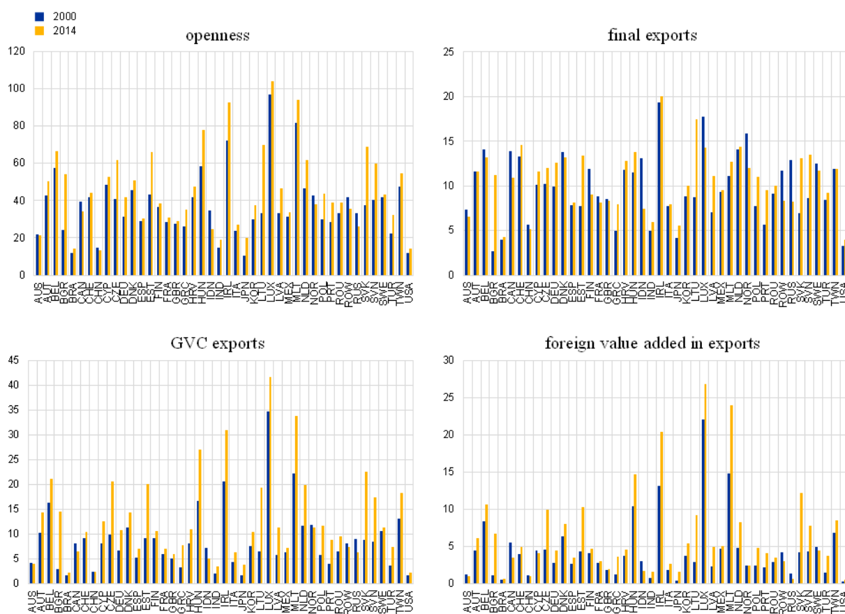
Figure 5: Changes in aggregate trade and global value chain participation
