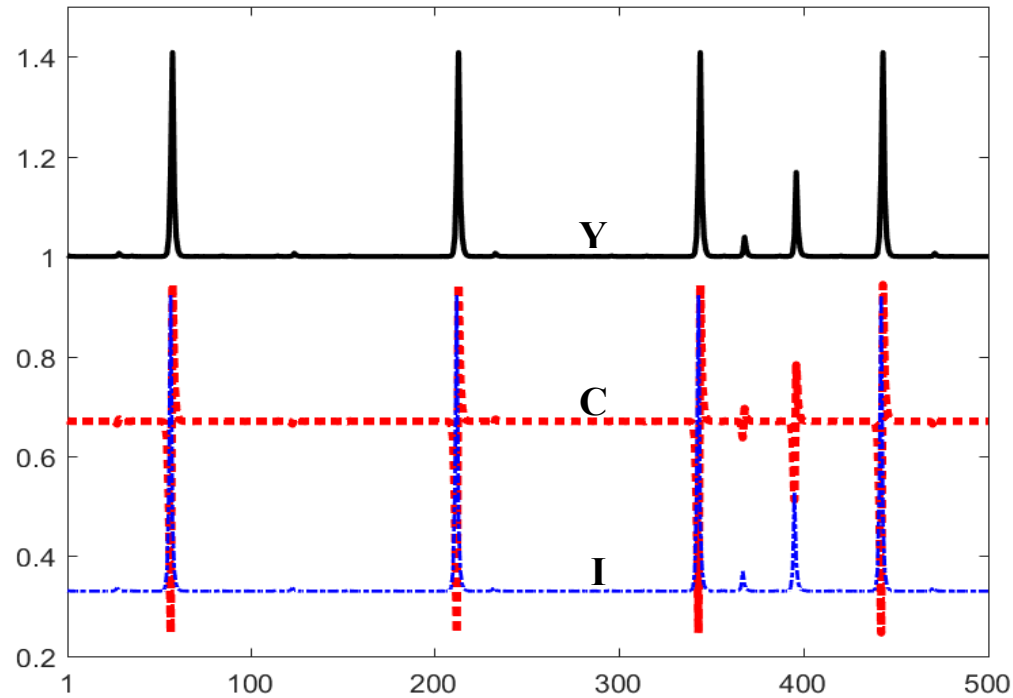
(2) Simulated paths
