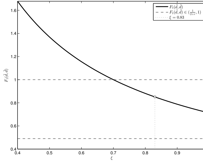
Figure 4: Stability Condition and the Intratemporal Elasticity of Substitution
