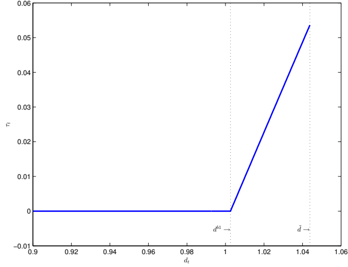
Figure 10: The Optimal Capital Control Policy
