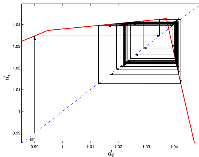
Figure 6: Convergence to a Two-Period Cycle: CES Aggregator
