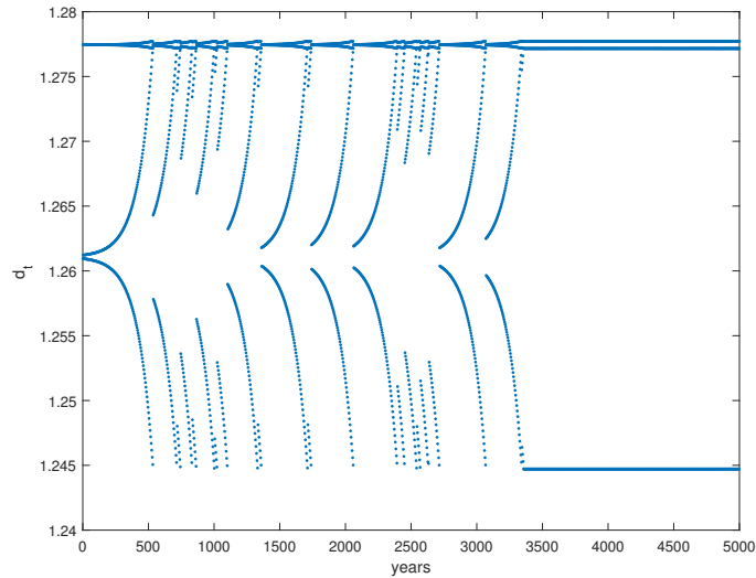
Figure 8: Convergence to a Three-Period Cycle: Cobb-Douglas Aggregator
