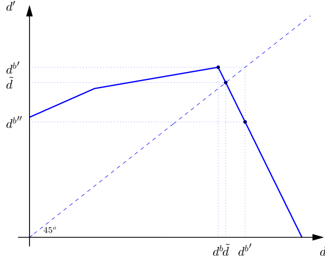
Figure 2: The Debt Policy Function with a Cobb-Douglas Aggregator
