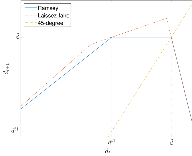
Figure 9: The Ramsey Optimal Debt Policy Function
