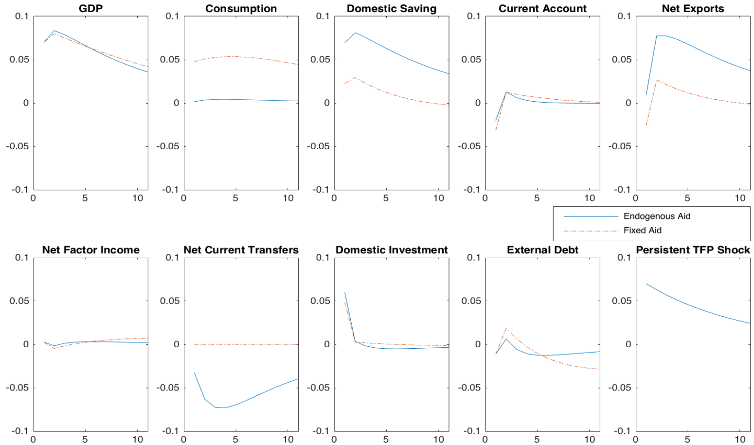
Figure 4 : Theoretical Impulse Responses to a Persistent Productivity Shock
