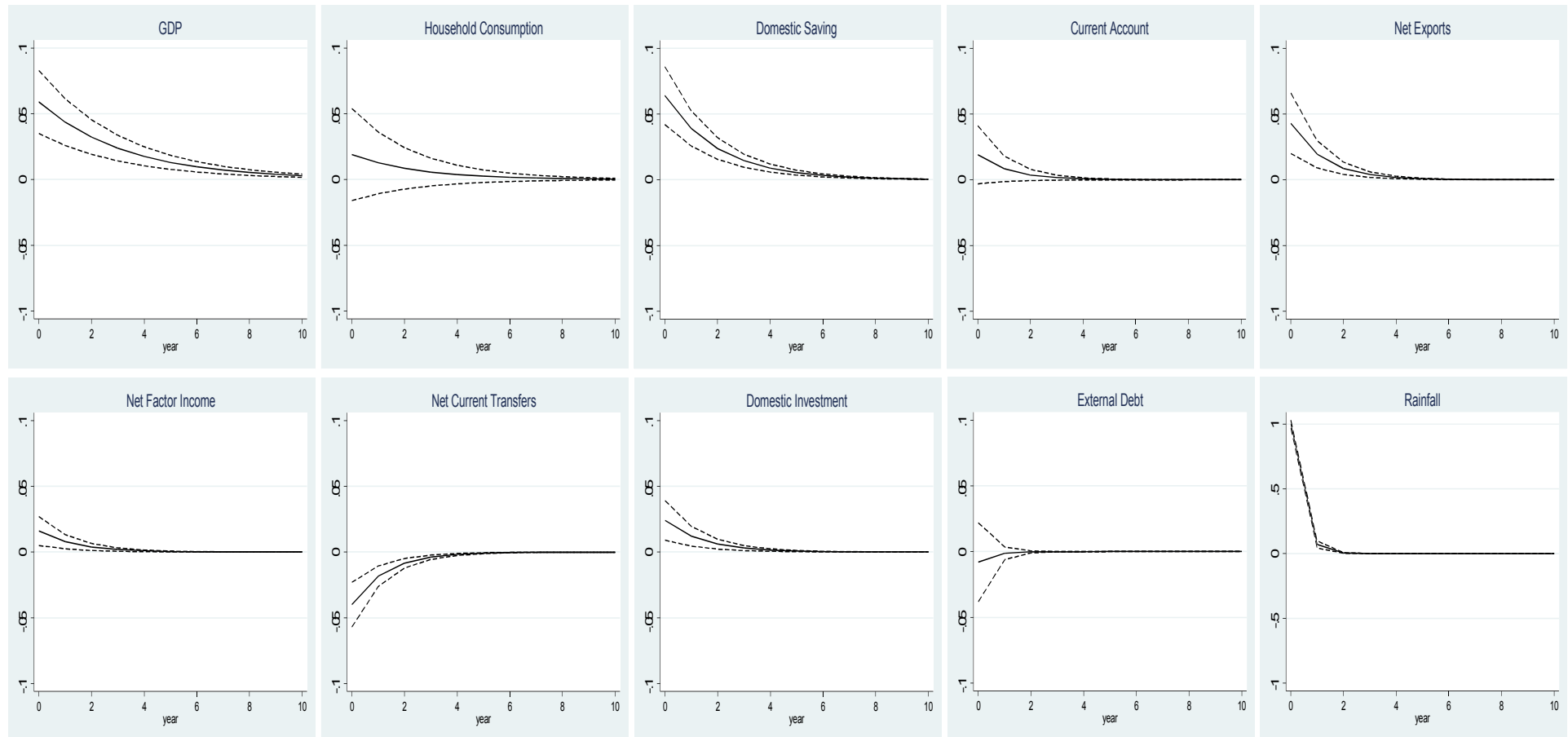
Figure 1. Empirical Impulse Responses to a Rainfall Shock
