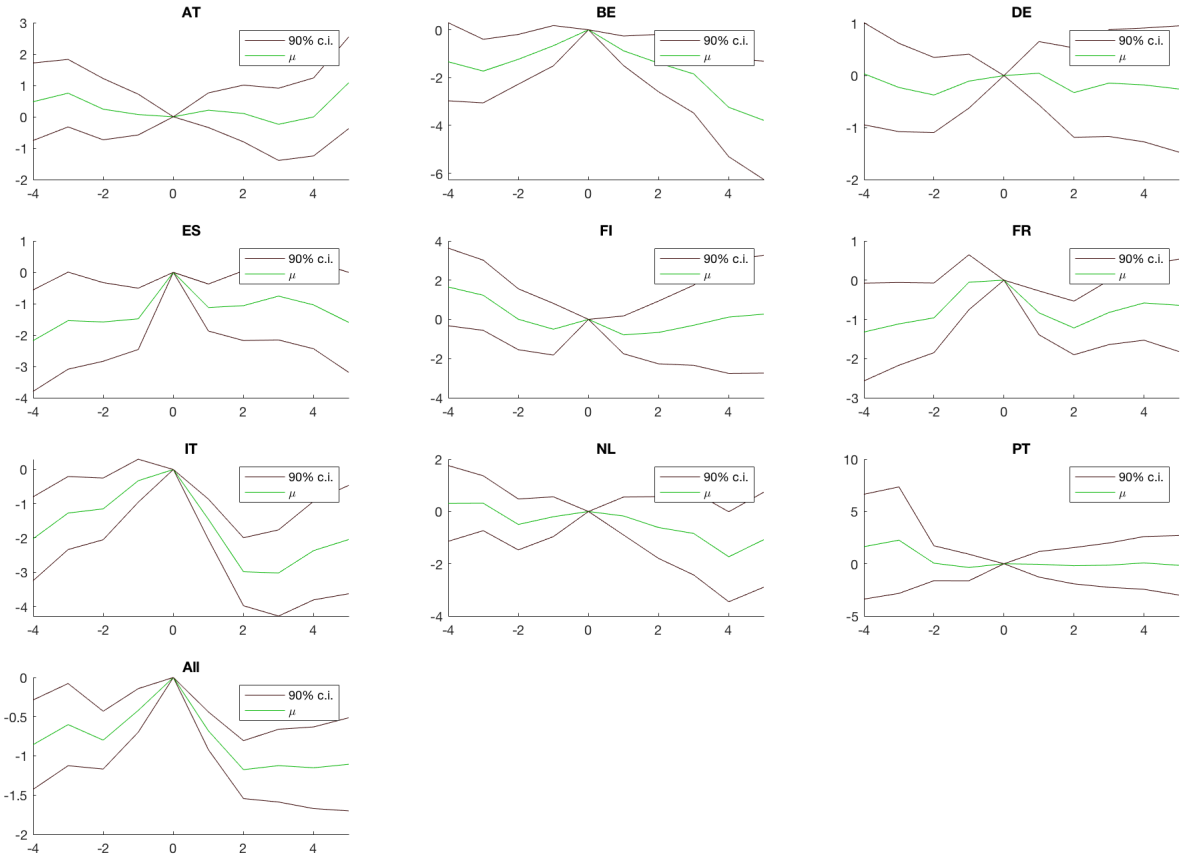
Figure 6: Event Study.
