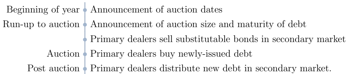
Figure 1: Auction Timeline.
