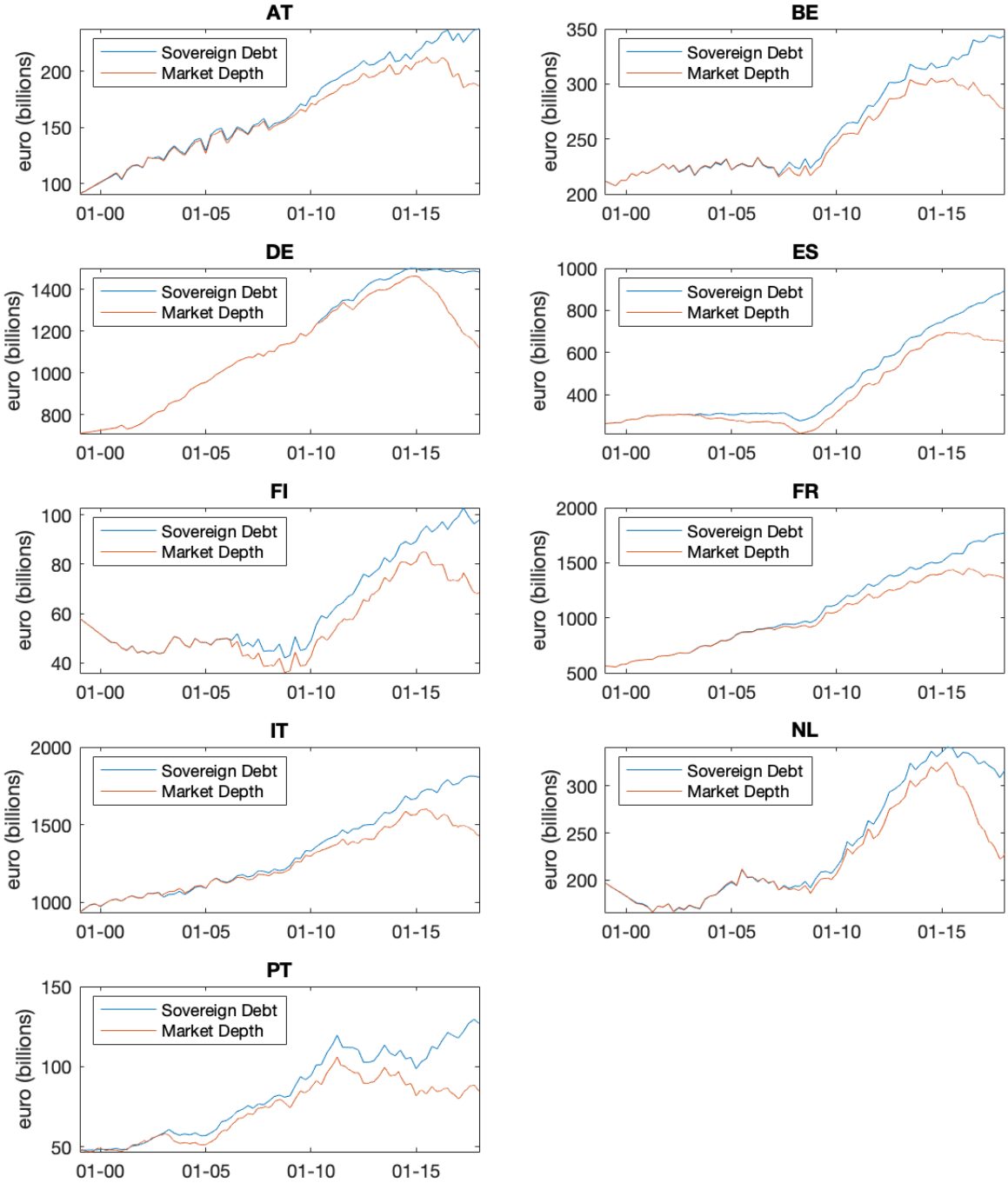
Figure 5: Market Depth
