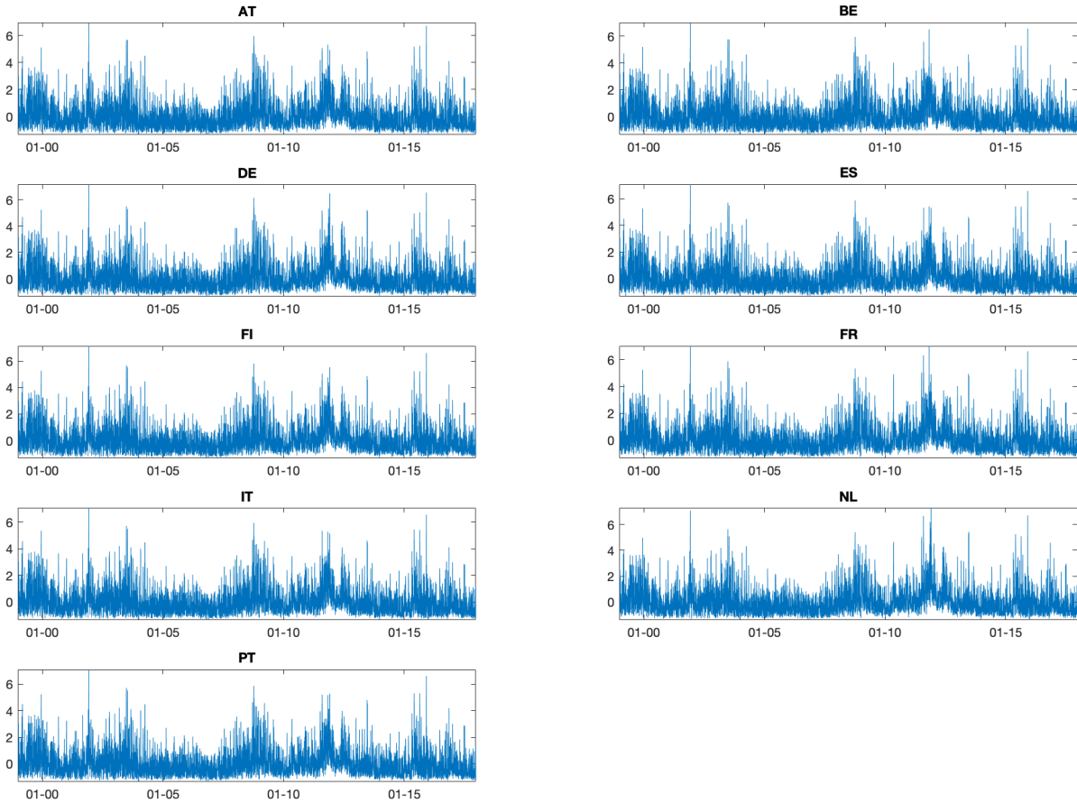
Figure 2: Market Volatility Factor.
