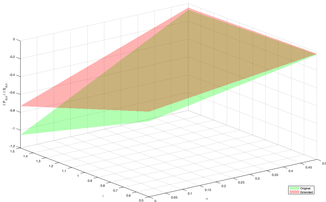
Figure 7: Numerical Results.
