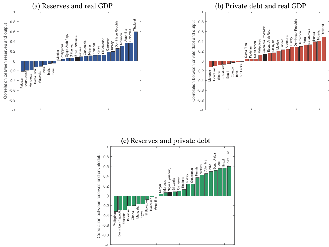
Figure 3: Correlation between the growth rates of real GDP and reserves (panel a), real GDP and private debt (panel b), and reserves and private debt (panel c)
