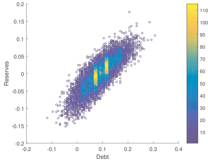
Figure 12: Increase in reserves and private debt
