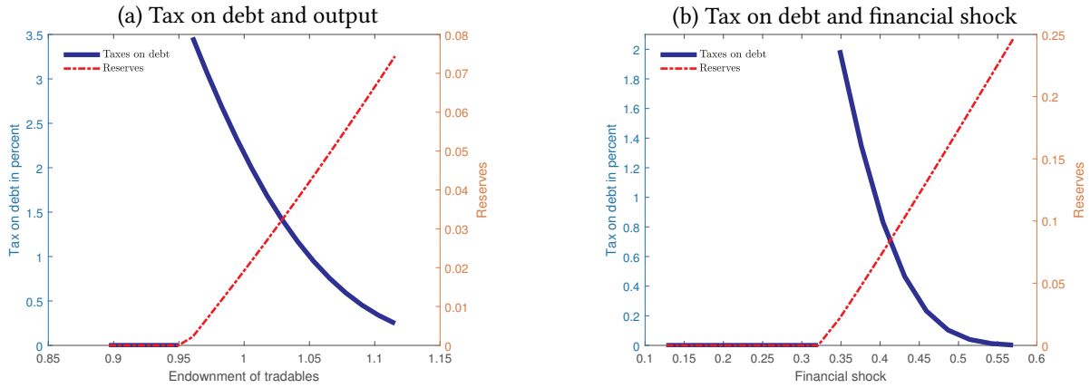
Figure 8: Policy functions: reserves vs. taxes
