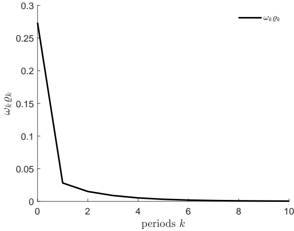
Figure 10: Correlation Decomposition
