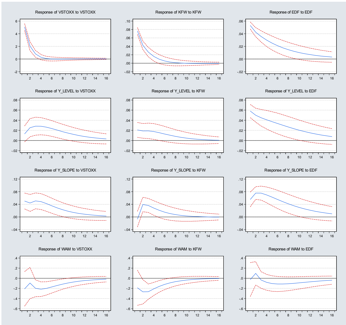
Figure 5: Impulse responses: core countries Belgium, France, Germany and Netherlands.
