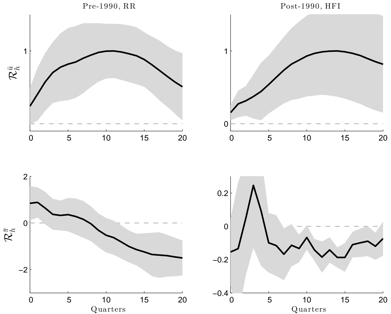
Figure 3: IRs of average inflation and unemployment — RR/HFI
