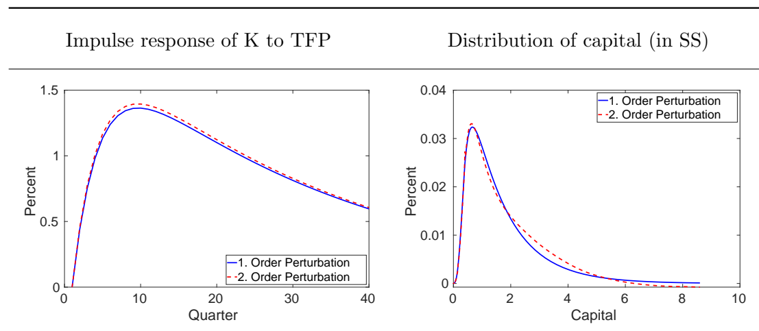
Figure 6: 2nd-order perturbation of Krusell-Smith model
